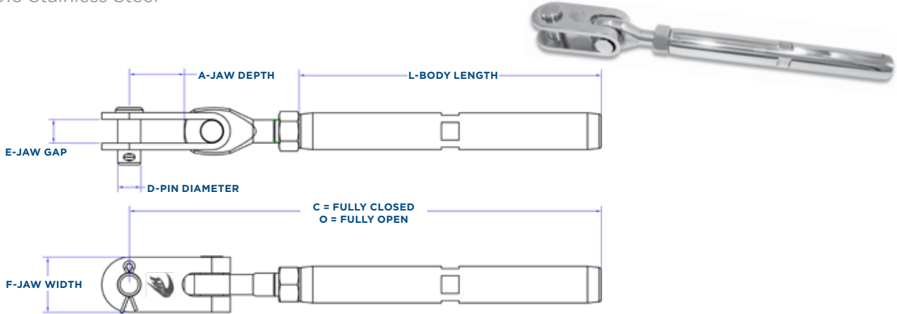
SMART PART # KEY eye toggle pin size | Eye Tubular Turnbuckle Jaw Toggle
