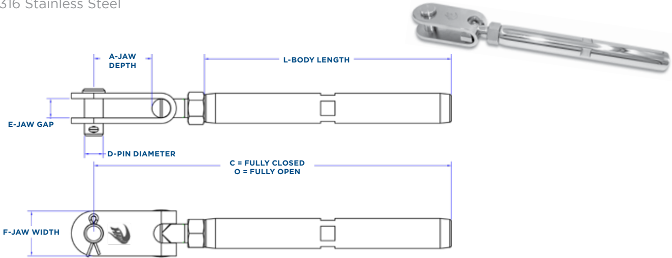
SMART PART # KEY toggle pin size | Tubular Turnbuckle Jaw Toggle
